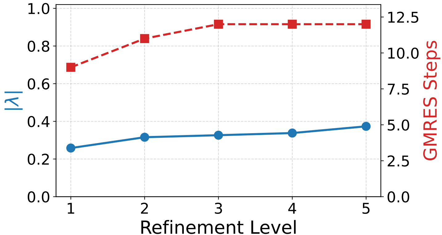
Magnetostatics: V-Cycle (Scaled Id)
