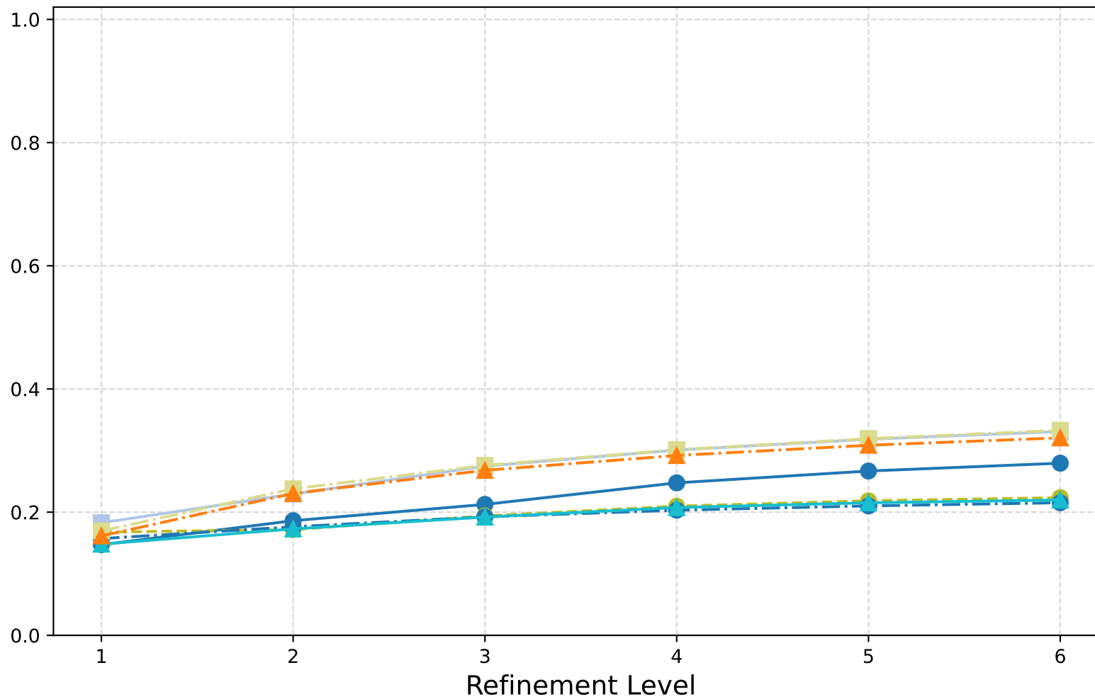
1-form Hodge Laplacian: V-Cycle (Scaled Id) - Spectral Radii
