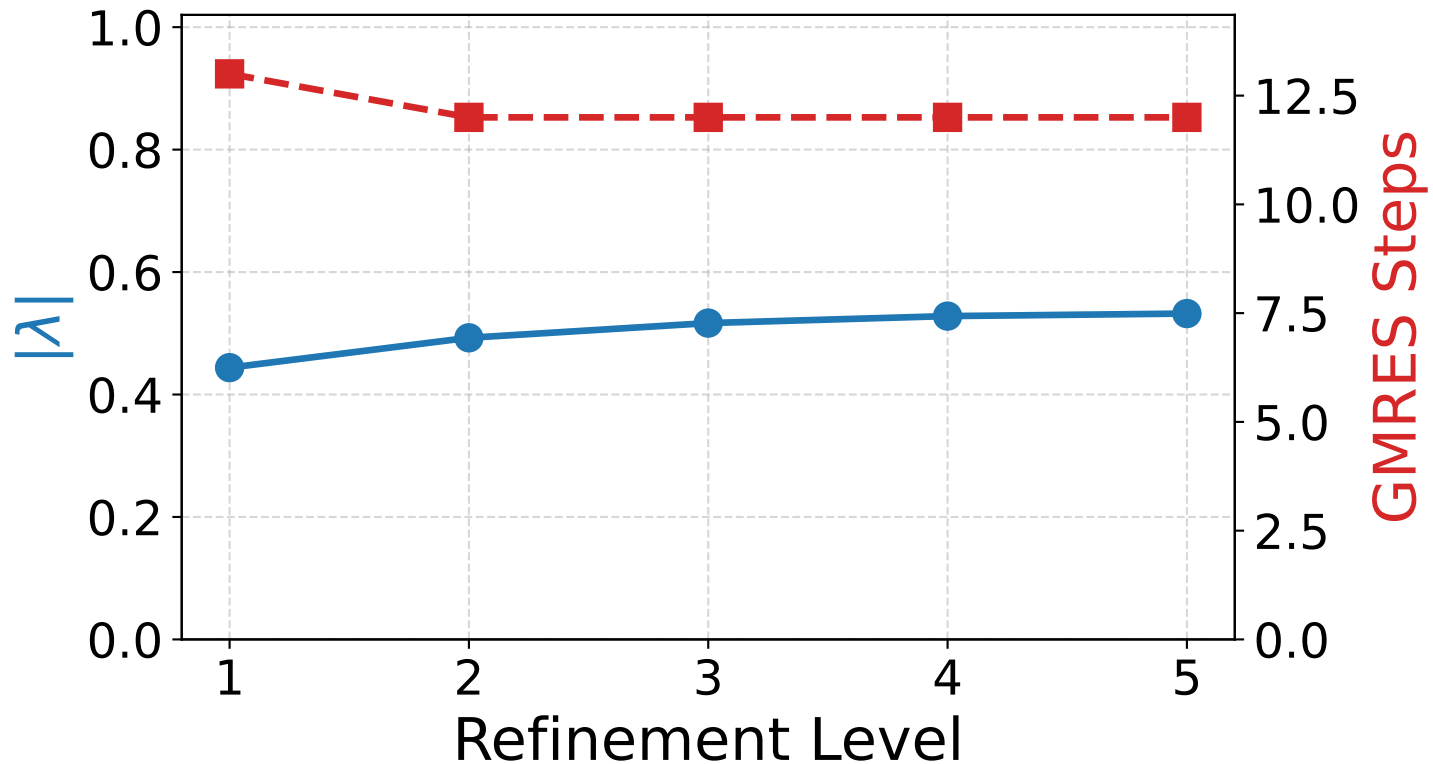
Dirac: W-Cycle (Scaled Id)
