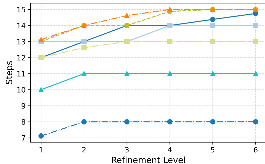
GMRES Iterations
