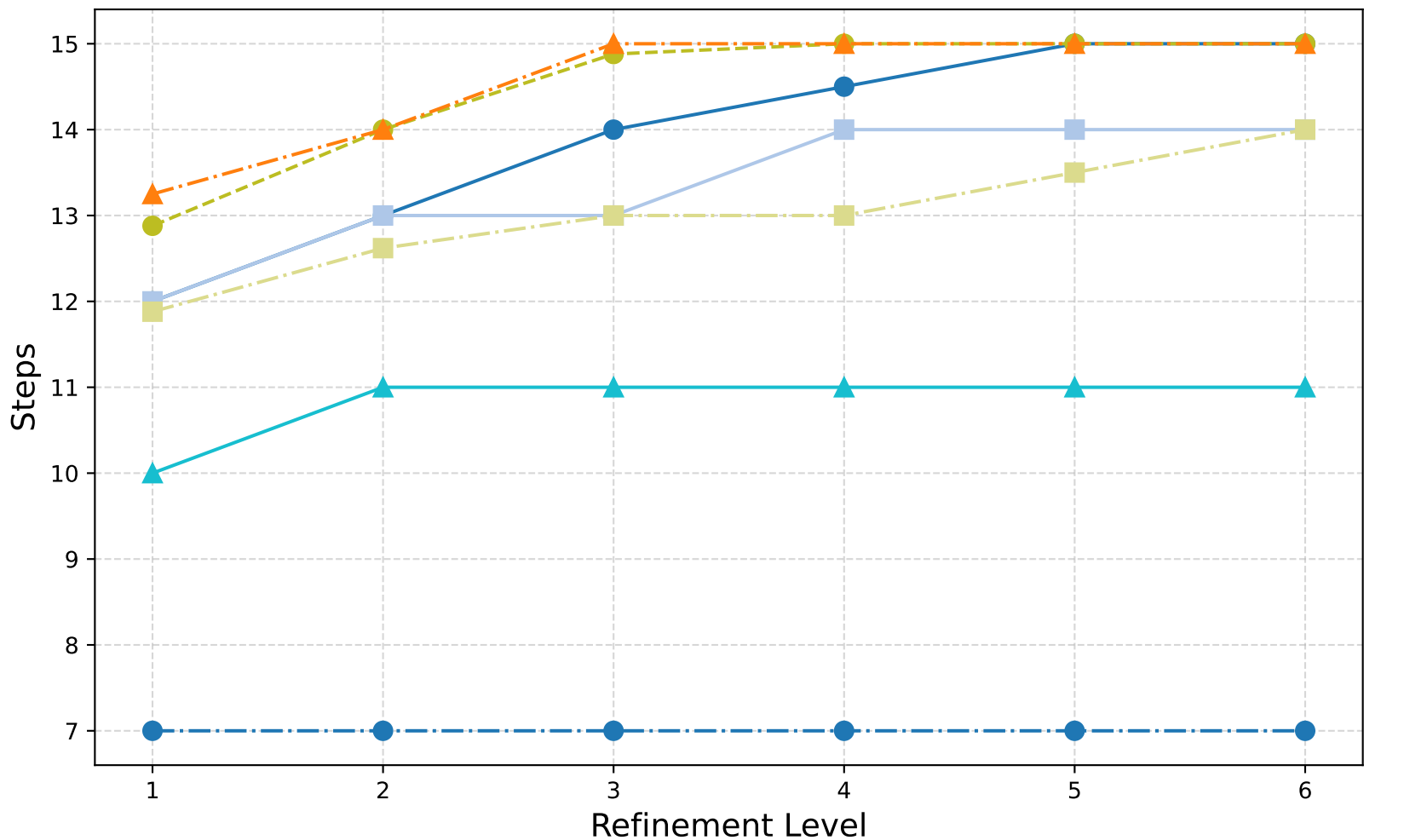
Magnetostatics: W-Cycle (Scaled Id) - GMRES Iterations
