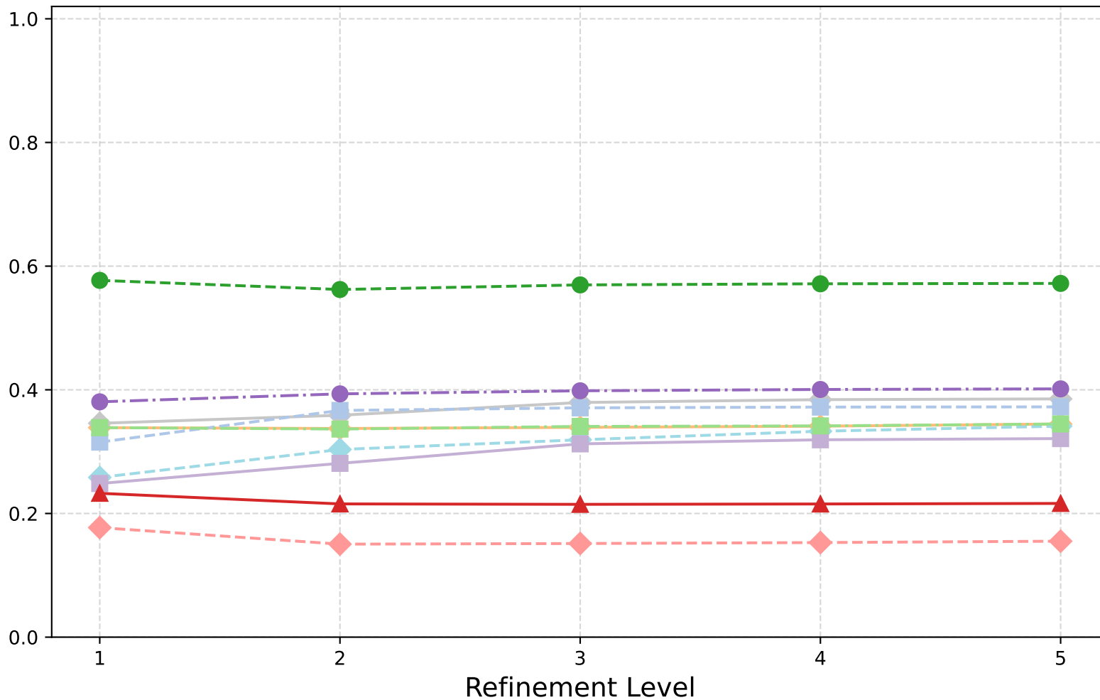
Magnetostatics: W-Cycle (Scaled Id) - Spectral Radii
