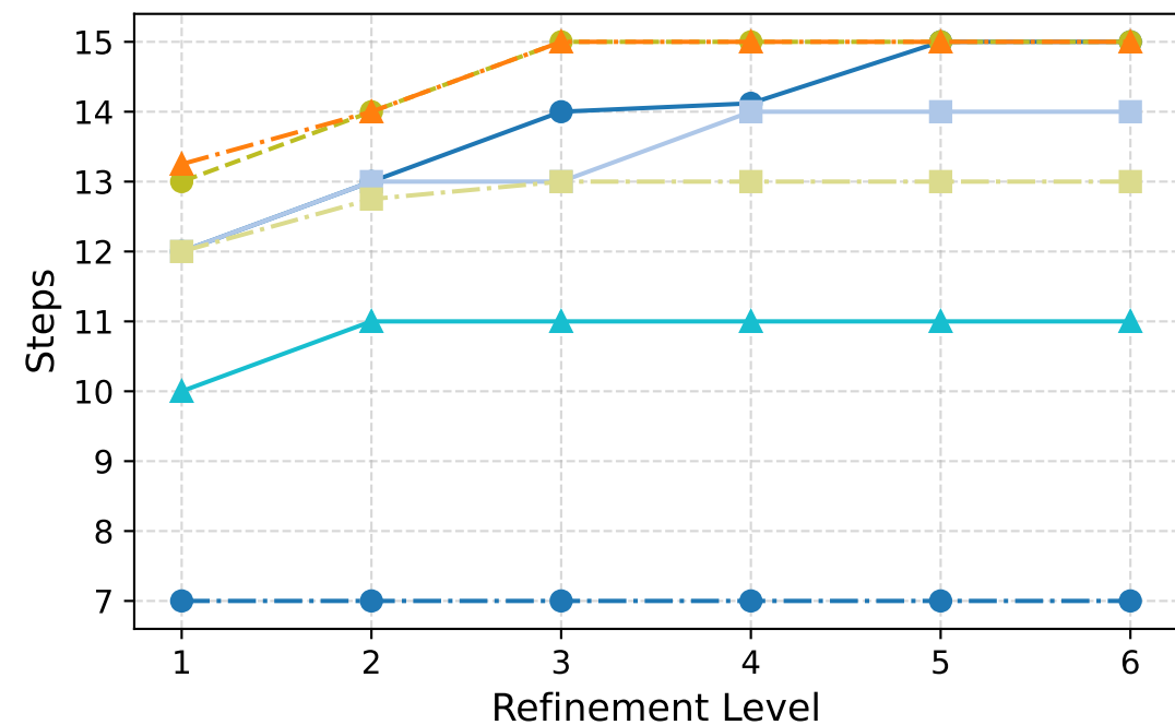
GMRES Iterations
