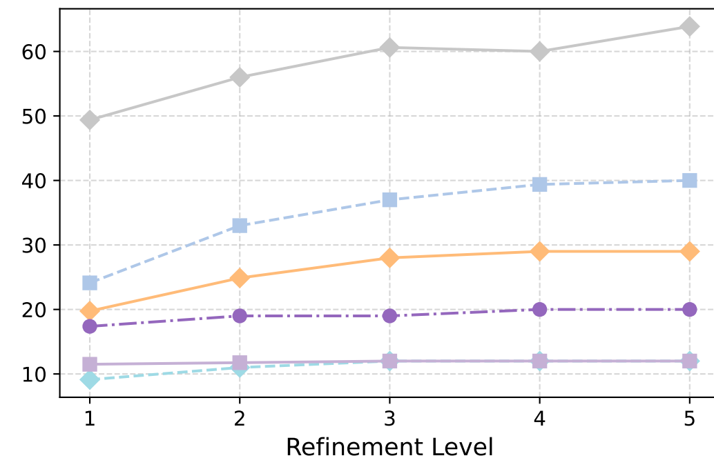
GMRES Iterations
