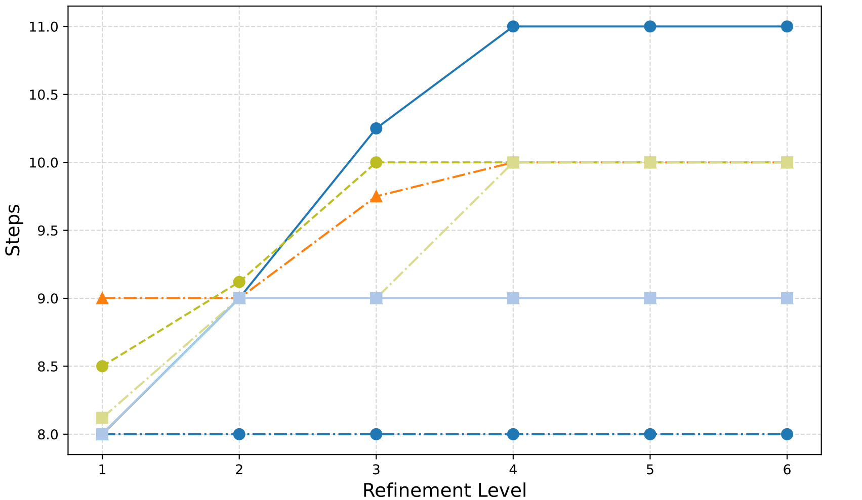
Dirac: V-Cycle (Barycentric) - GMRES Iterations
