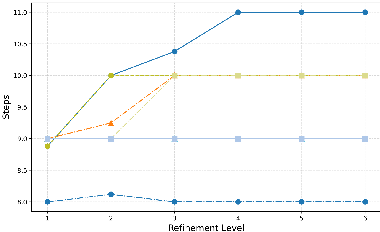
HCurl Laplacian: V-Cycle (Barycentric) - GMRES Iterations
