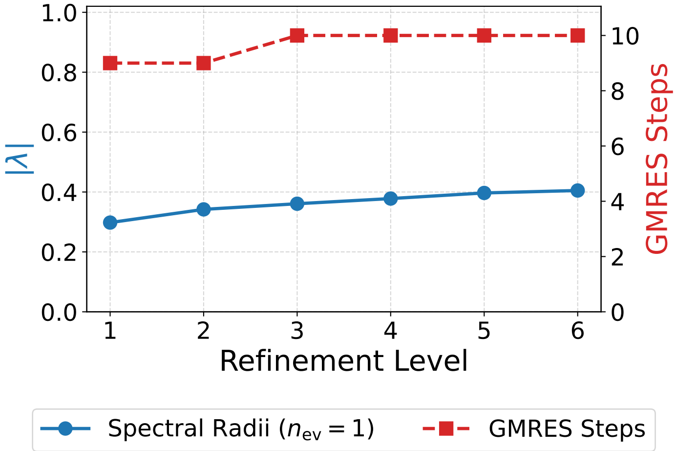
HCurl Laplacian: V-Cycle (Barycentric)
