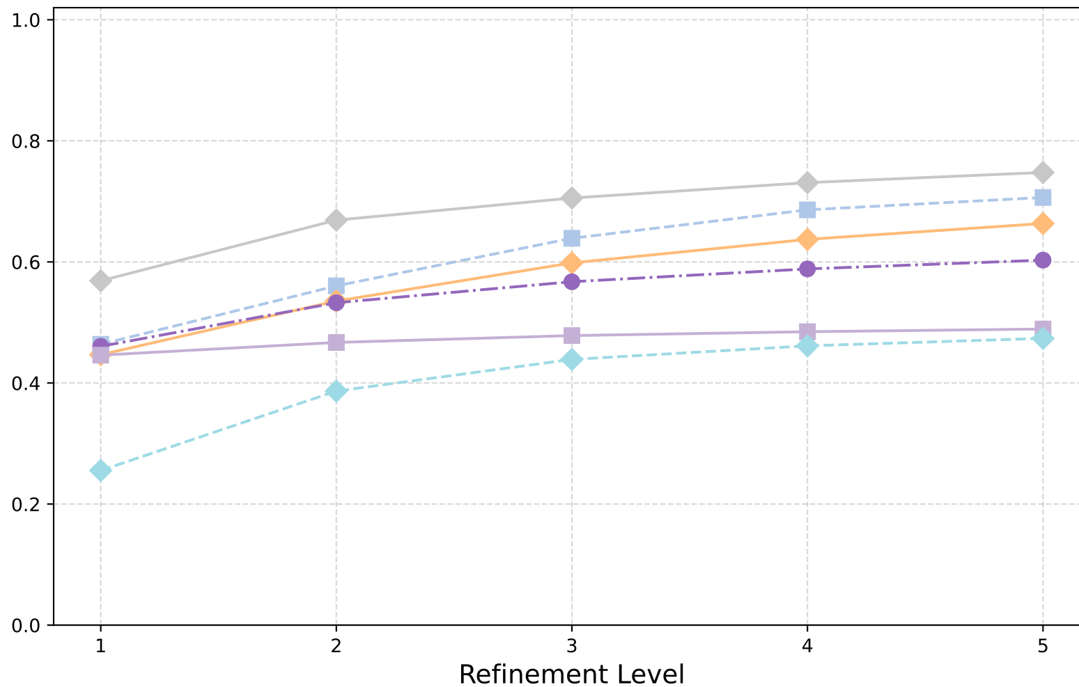
HCurl Laplacian: V-Cycle (Barycentric) - Spectral Radii
