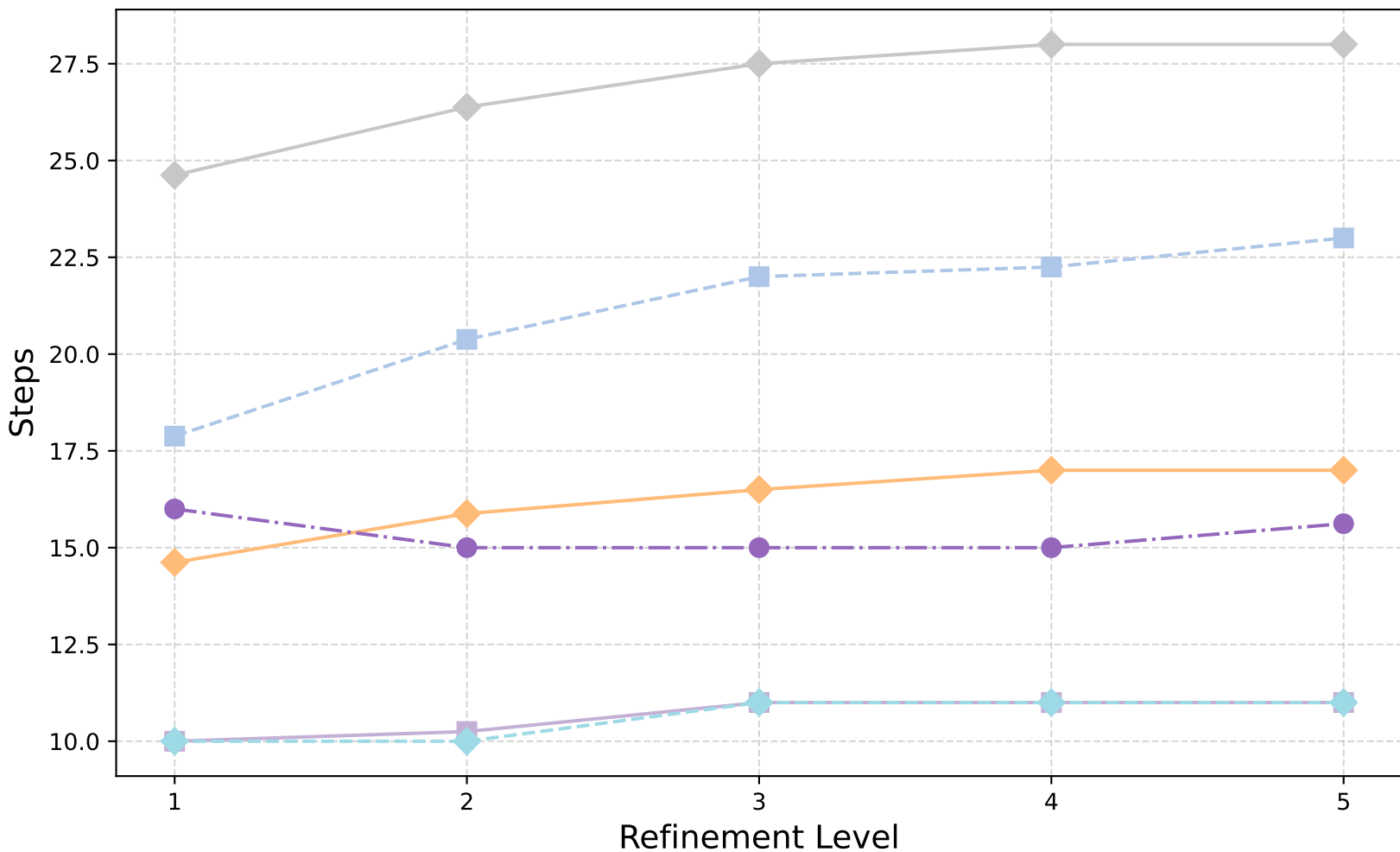
Dirac: W-Cycle (Barycentric) - GMRES Iterations
