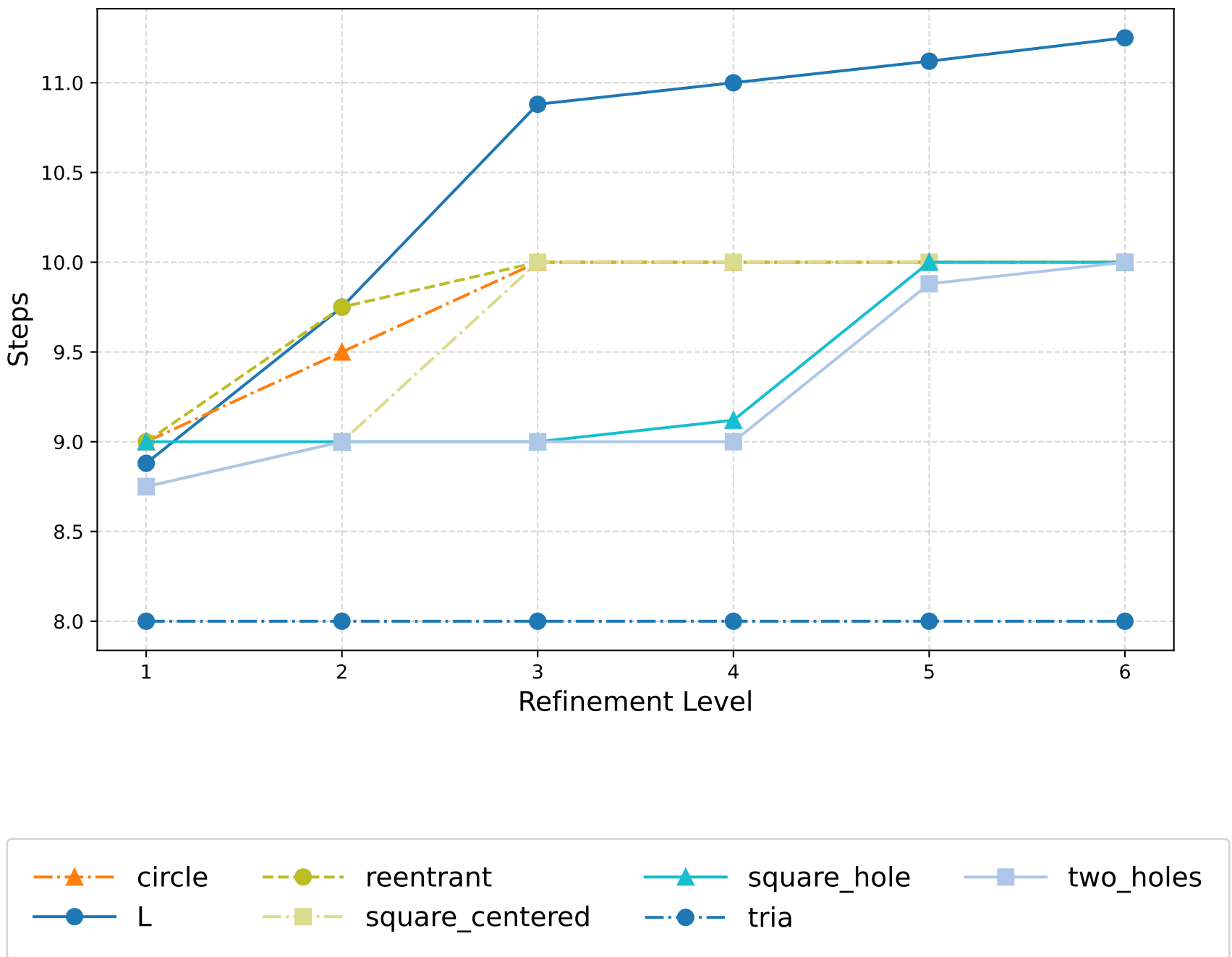
Magnetostatics: W-Cycle (Barycentric) - GMRES Iterations
