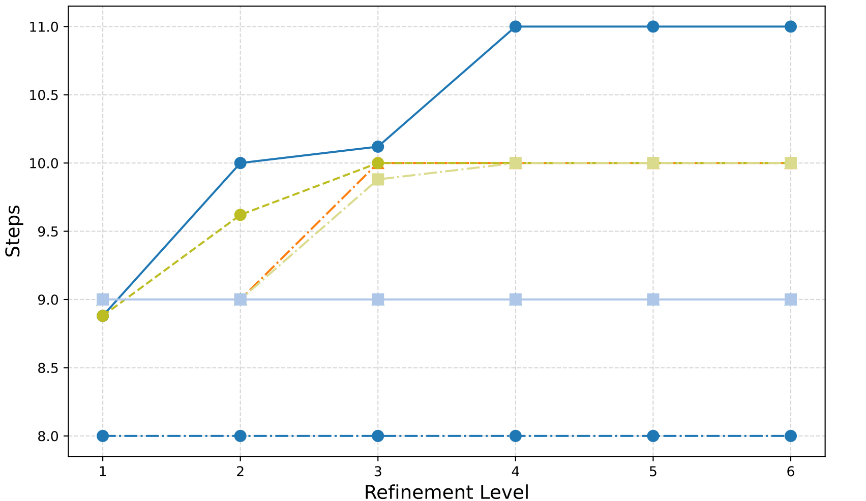
HCurl Laplacian: W-Cycle (Barycentric) - GMRES Iterations
