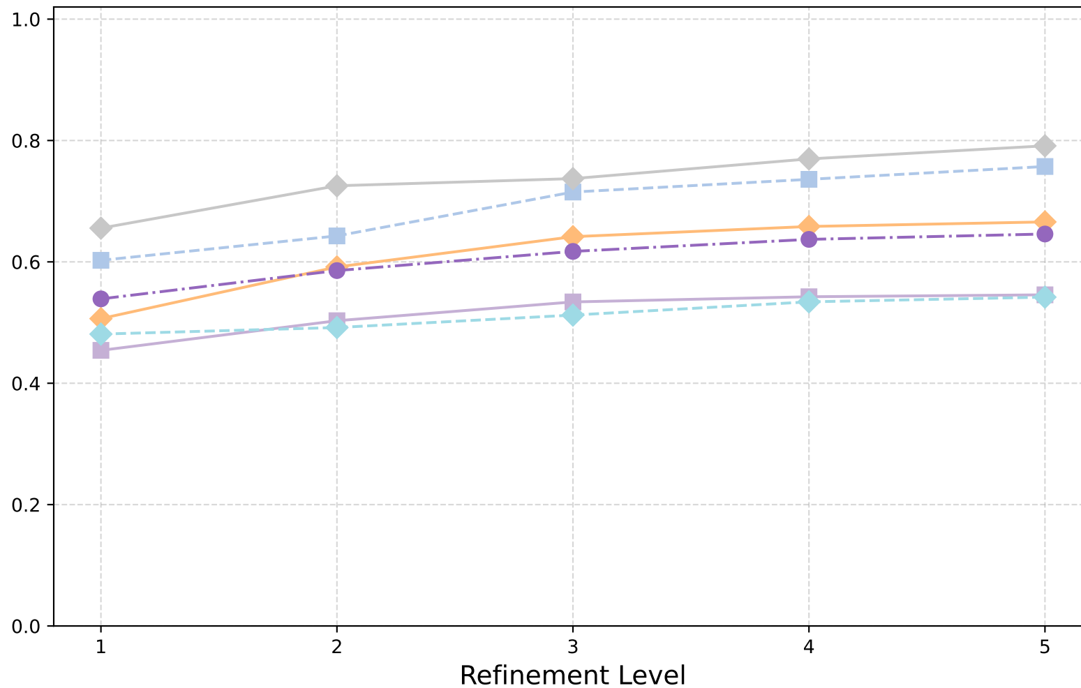
Dirac: V-Cycle (Row Sum) - Spectral Radii
