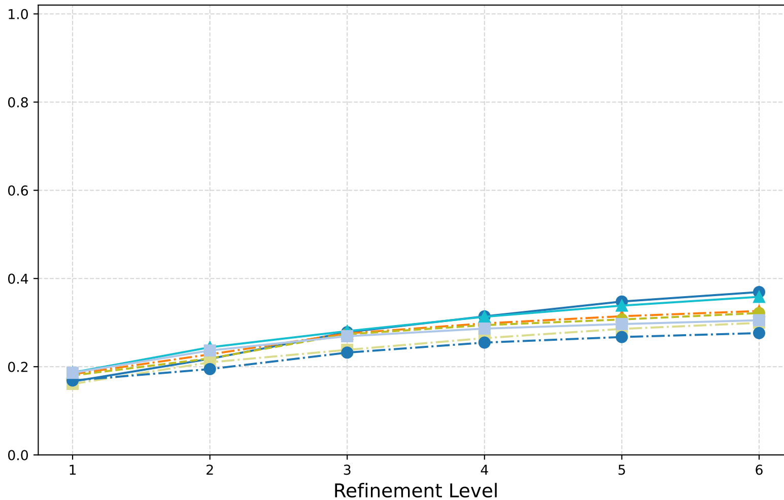
Magnetostatics: V-Cycle (Row Sum) - Spectral Radii
