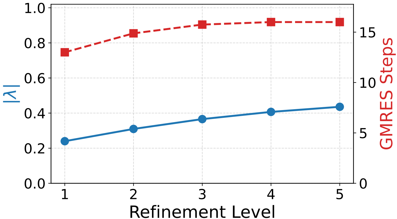
Magnetostatics: V-Cycle (Row Sum)
