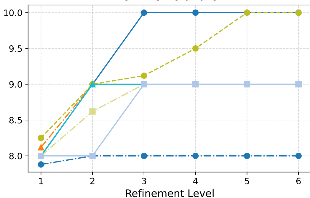
GMRES Iterations
