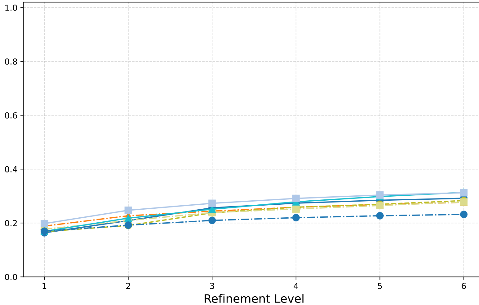
HxCurl Laplacian: V-Cycle (Row Sum) - Spectral Radii
