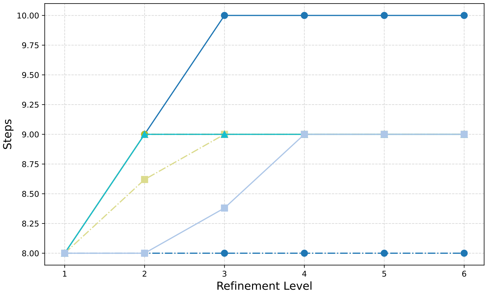
HCurl Laplacian: V-Cycle (Row Sum) - GMRES Iterations
