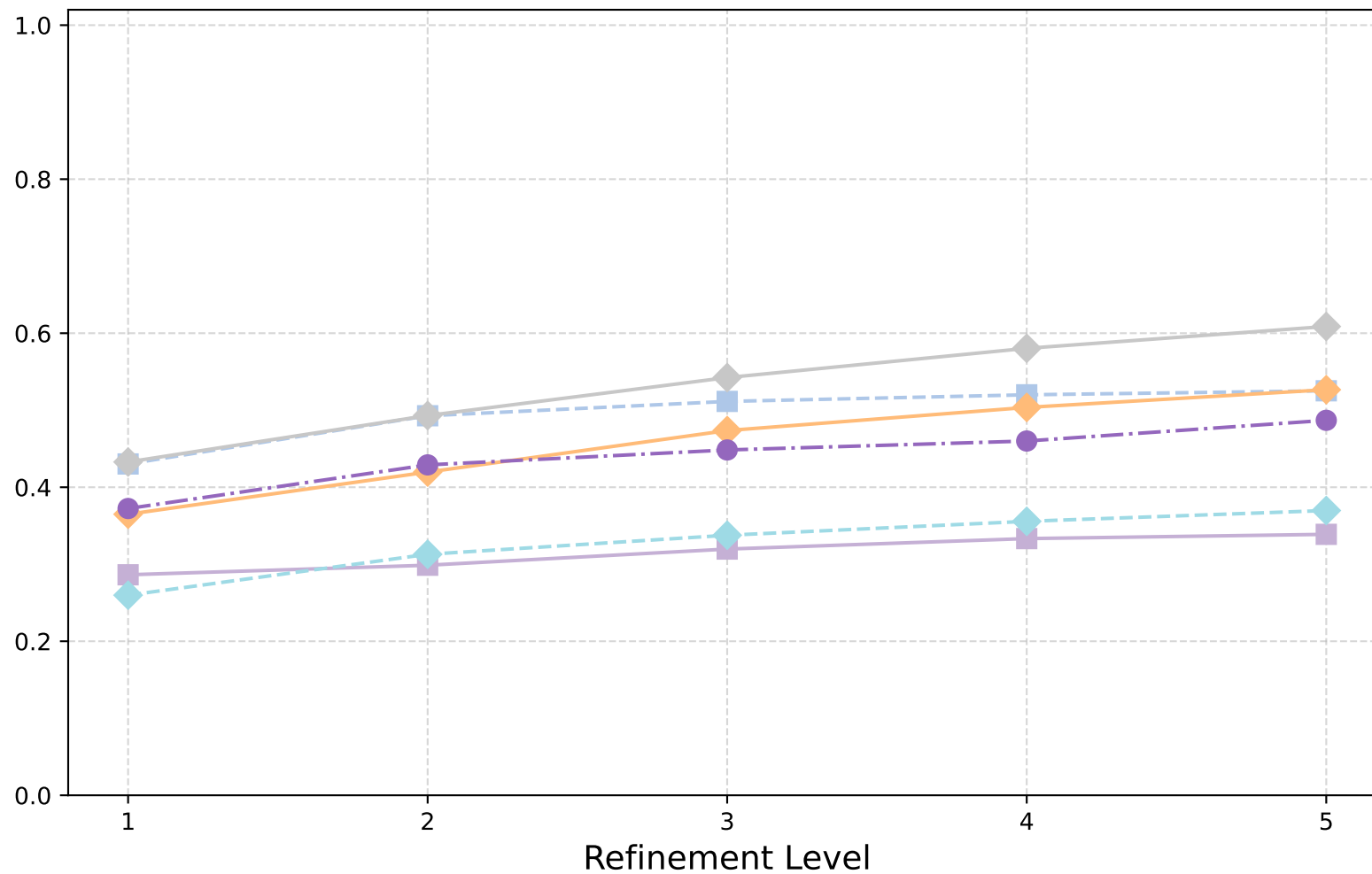
HCurl Laplacian: V-Cycle (Row Sum) - Spectral Radii
