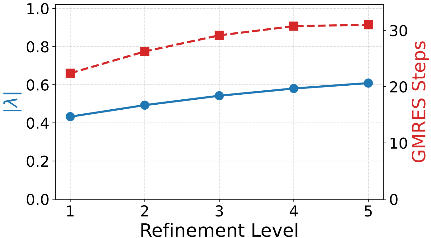
H Curl Laplacian: V-Cycle (Row Sum)
