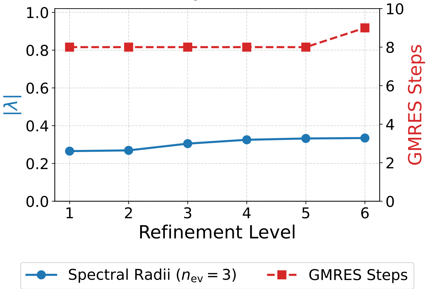
Dirac: W-Cycle (Row Sum)
