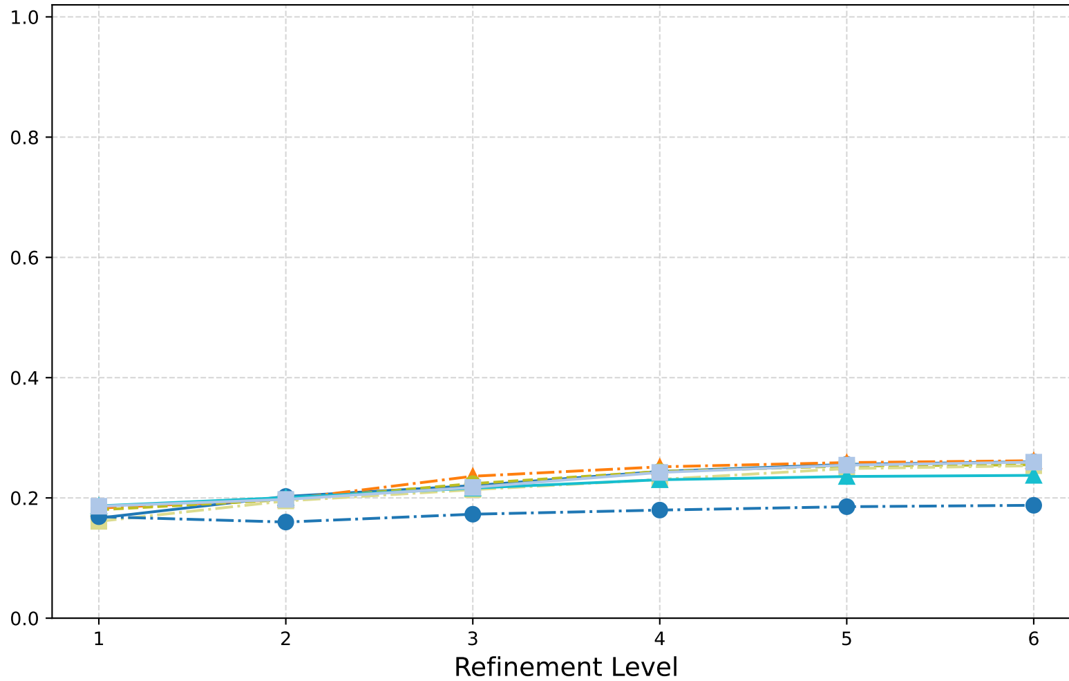
Magnetostatics: W-Cycle (Row Sum) - Spectral Radii
