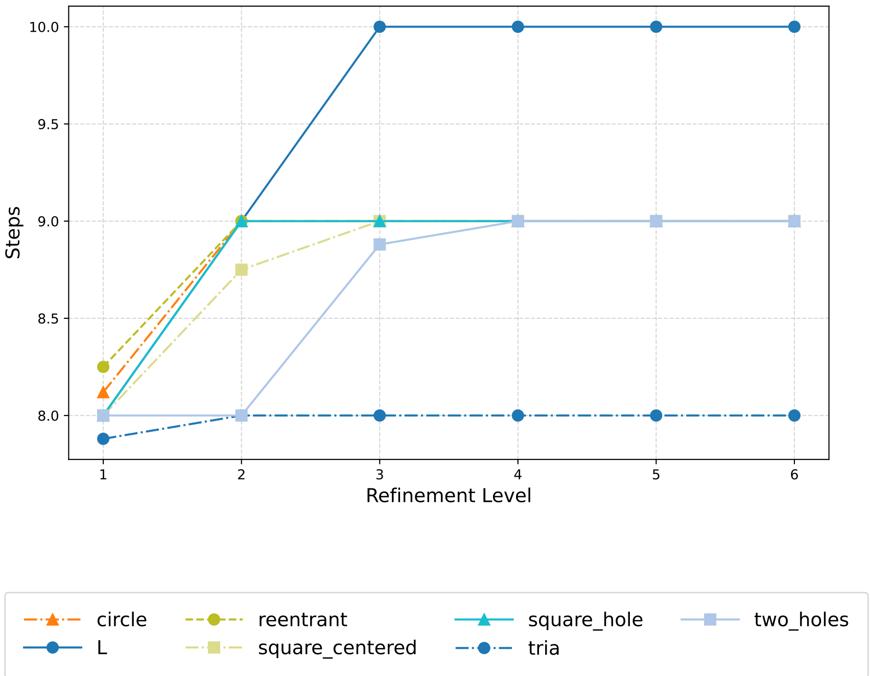
Magnetostatics: W-Cycle (Row Sum) - GMRES Iterations
