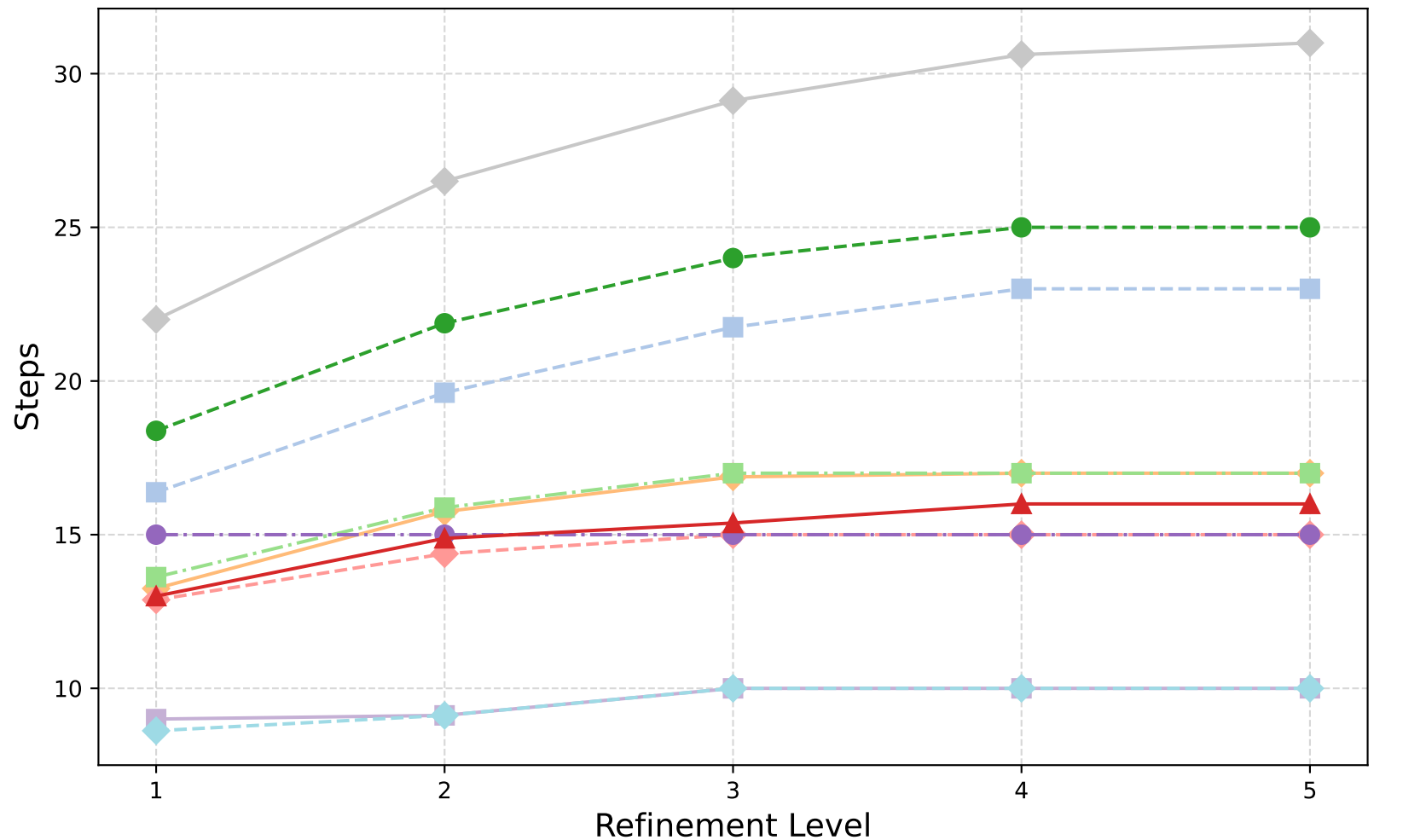
Magnetostatics: W-Cycle (Row Sum) - GMRES Iterations
