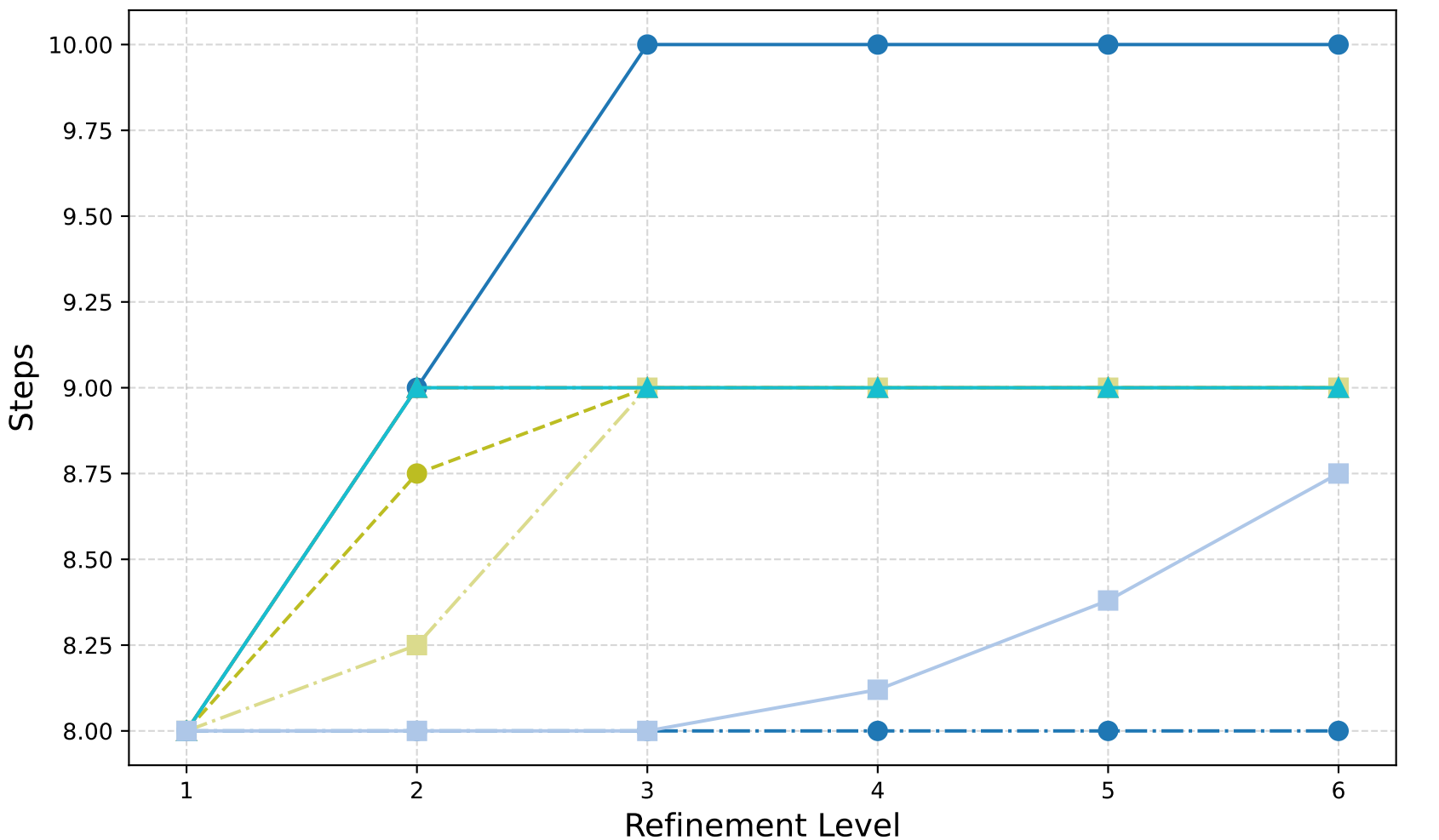
HCurl Laplacian: W-Cycle (Row Sum) - GMRES Iterations
