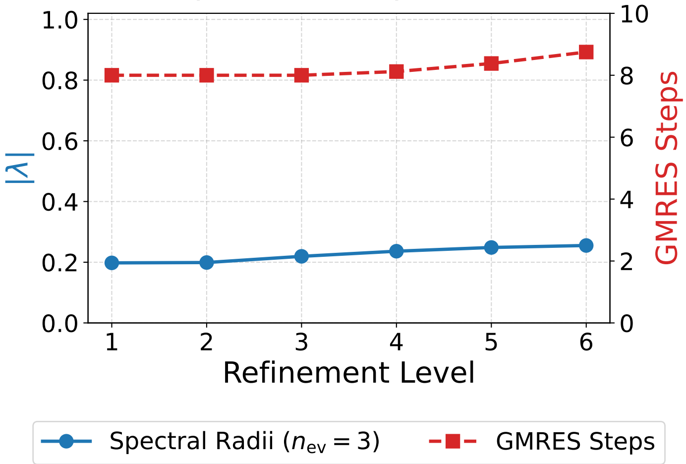
HCurl Laplacian: W-Cycle (Row Sum)
