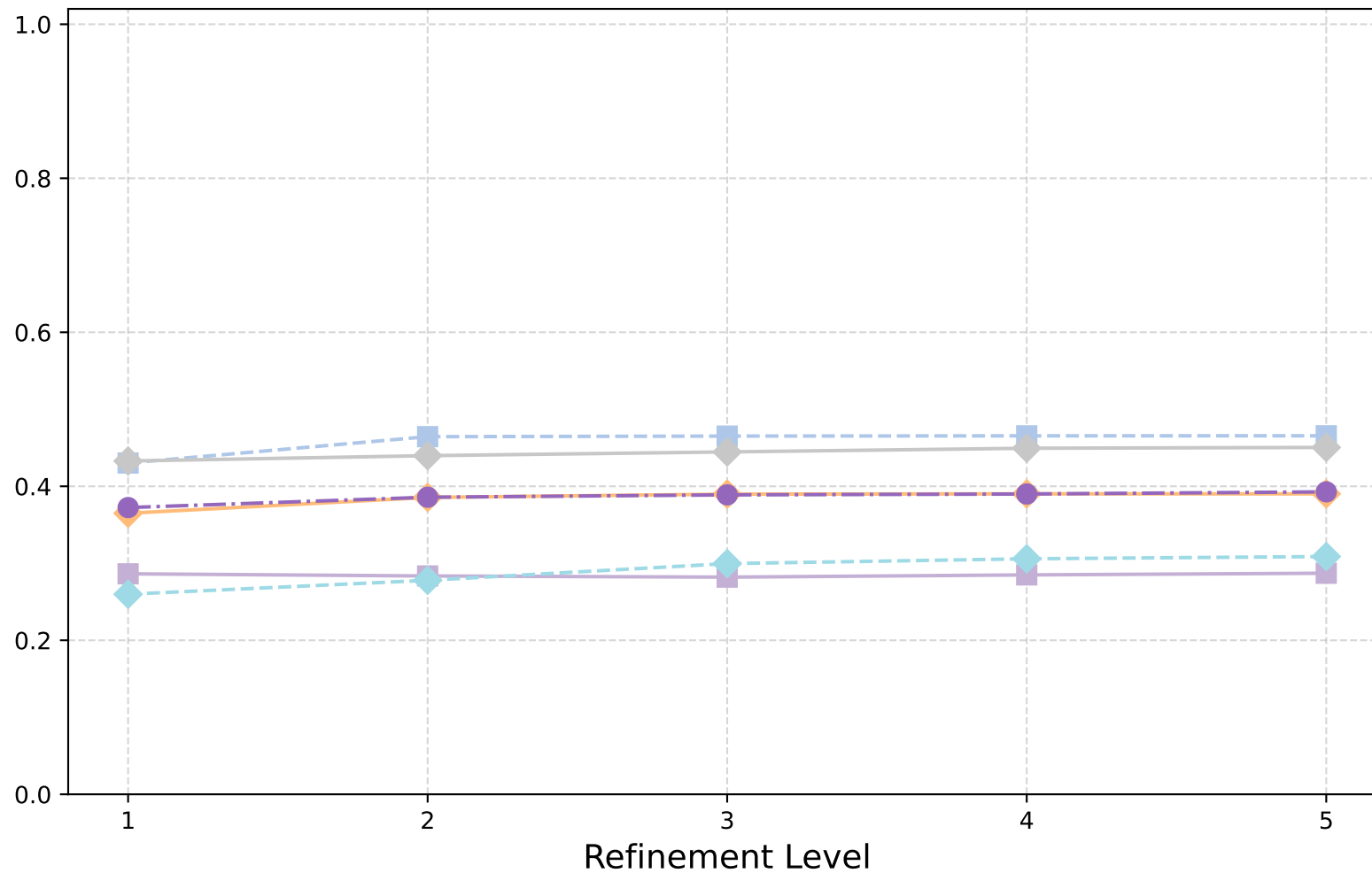
HCurl Laplacian: W-Cycle(Row Sum) - Spectral Radii
