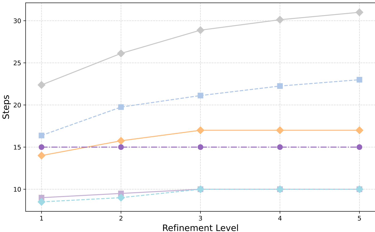
HCurl Laplacian: W-Cycle (Row Sum) - GMRES Iterations
