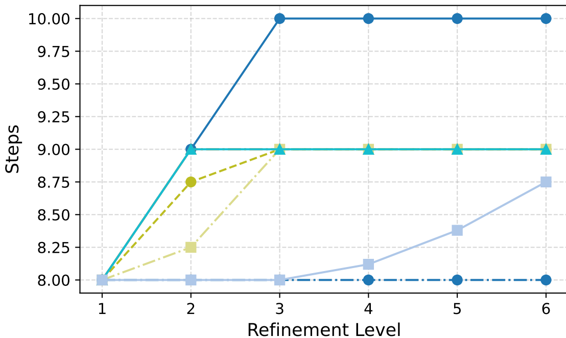
GMRES Iterations
