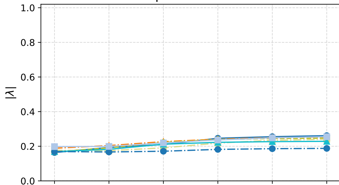
Spectral Radii
