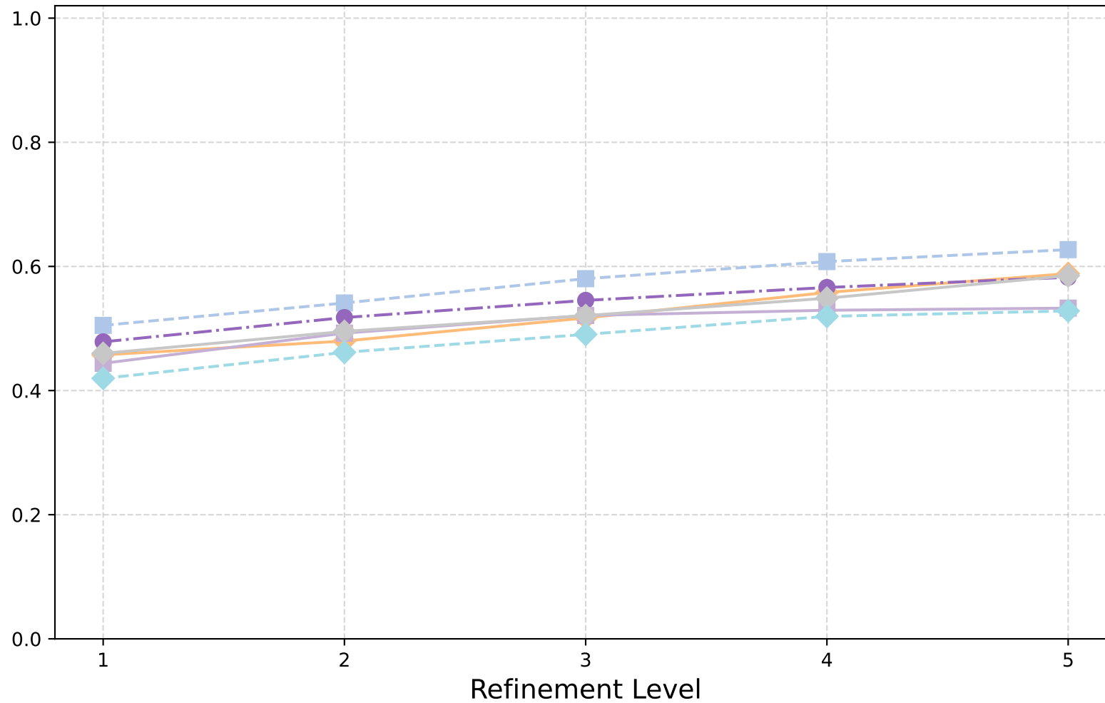
Dirac: V-Cycle (Scaled Id) - Spectral Radii
