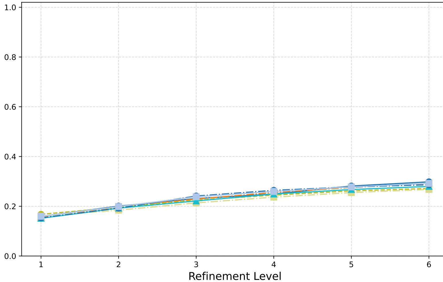
Magnetostatics: V-Cycle (Scaled Id) - Spectral Radii
