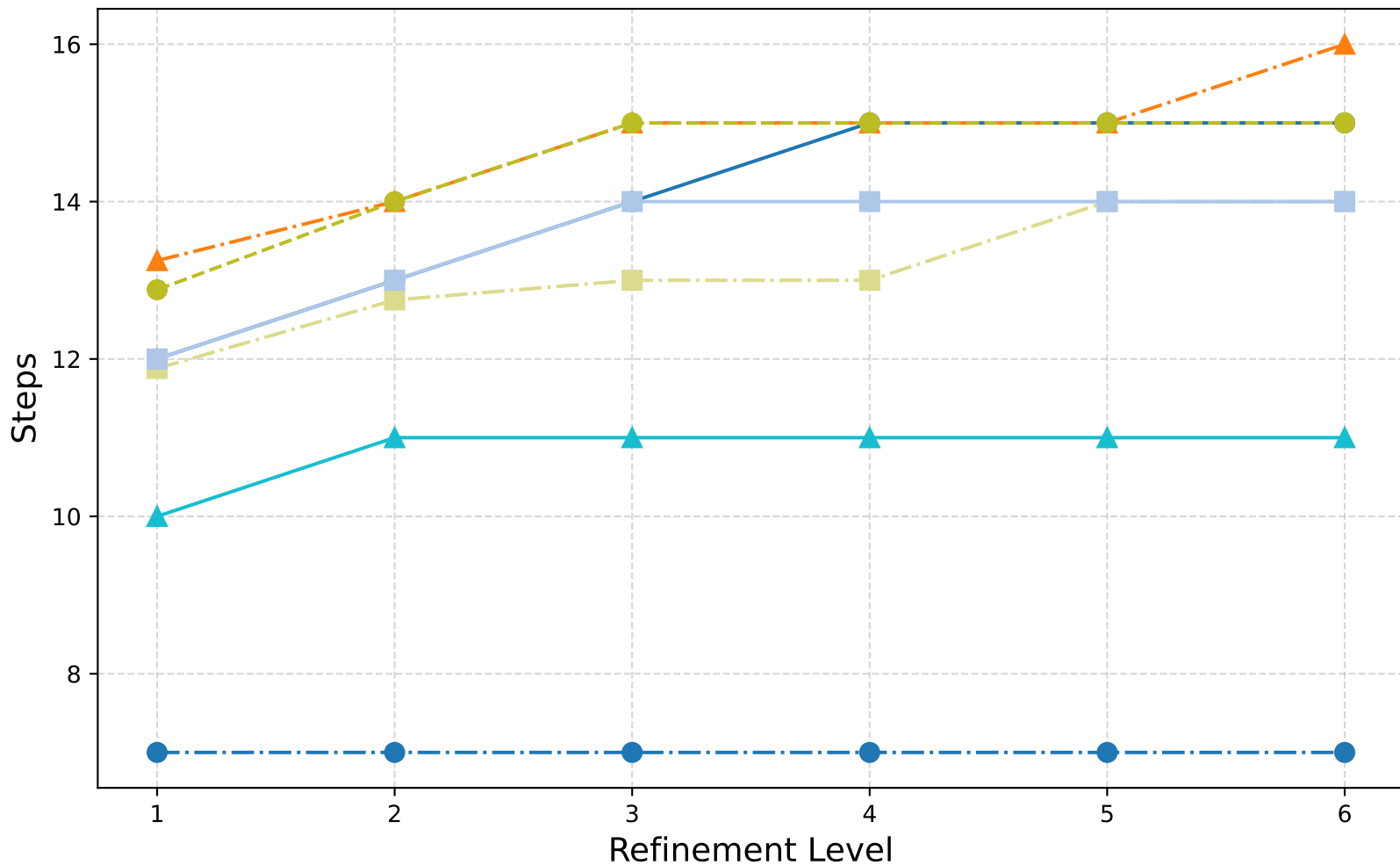
Magnetostatics: V-Cycle (Scaled Id) - GMRES Iterations
