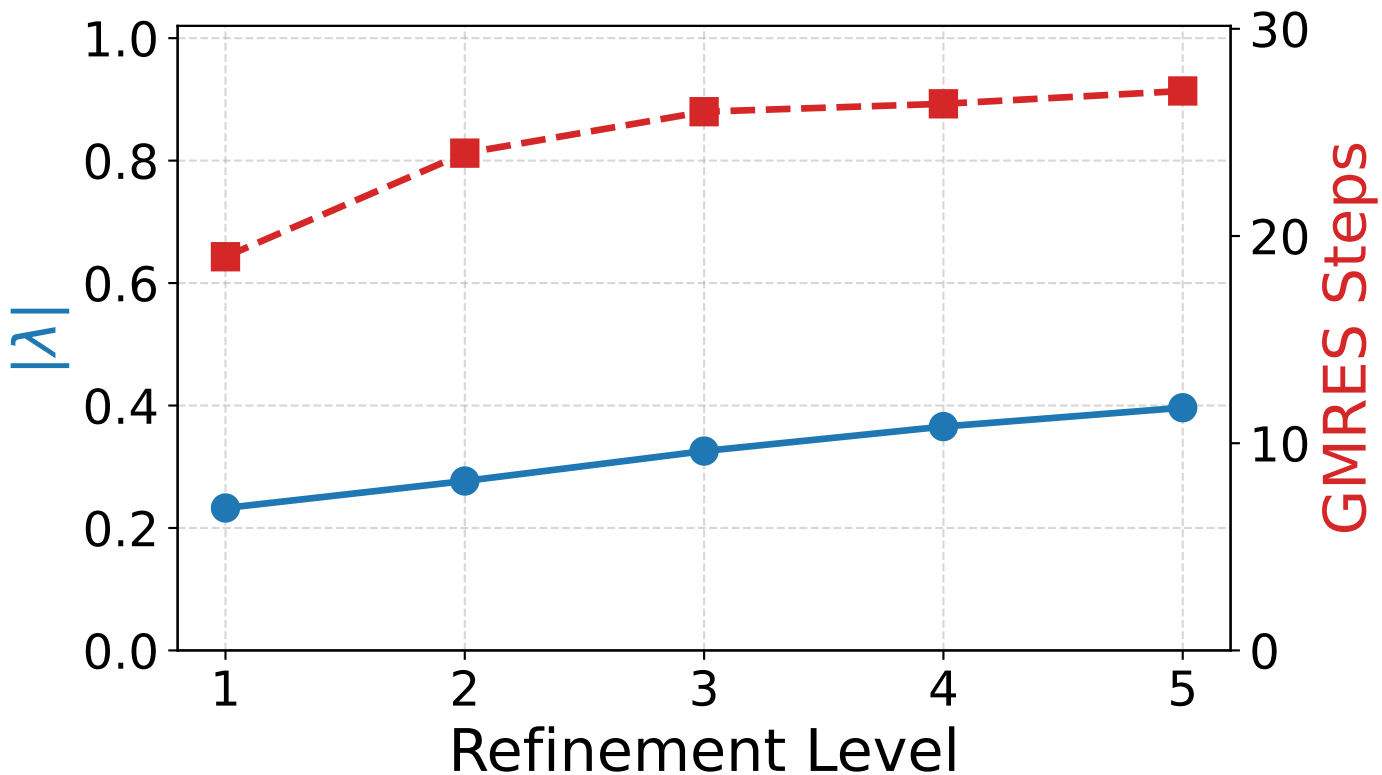
Magnetostatics: V-Cycle (Scaled Id)
