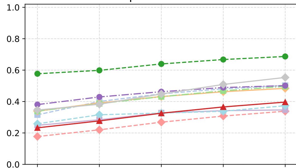
Spectral Radii
