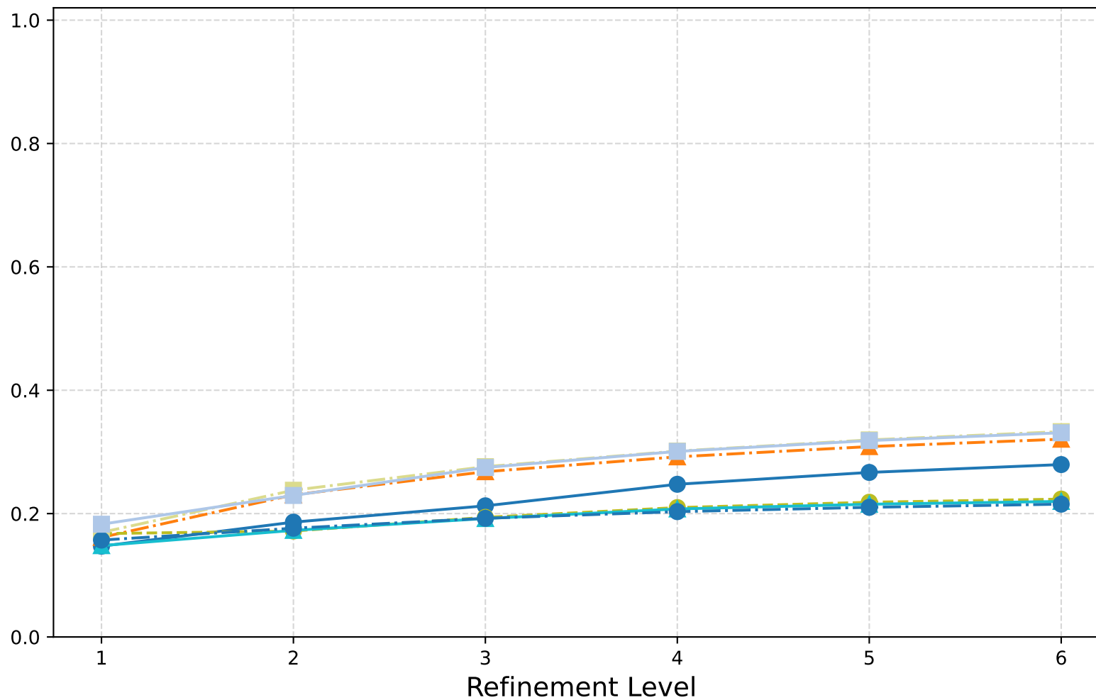
H Curl Laplacian: V-Cycle (Scaled Id) - Spectral Radii
