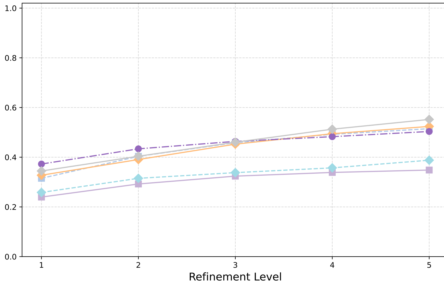
HCurl Laplacian: V-Cycle (Scaled Id) - Spectral Radii
