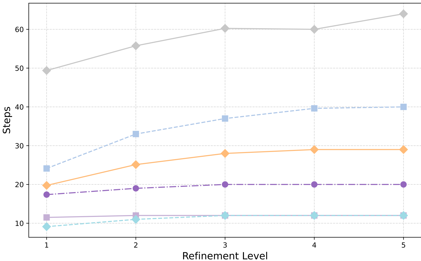
HCurl Laplacian: V-Cycle (Scaled Id) - GMRES Iterations
