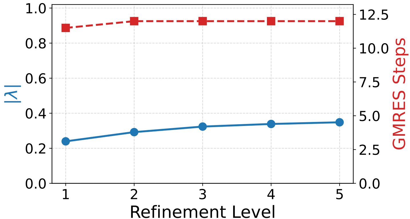
HCurl Laplacian: V-Cycle (Scaled Id)
