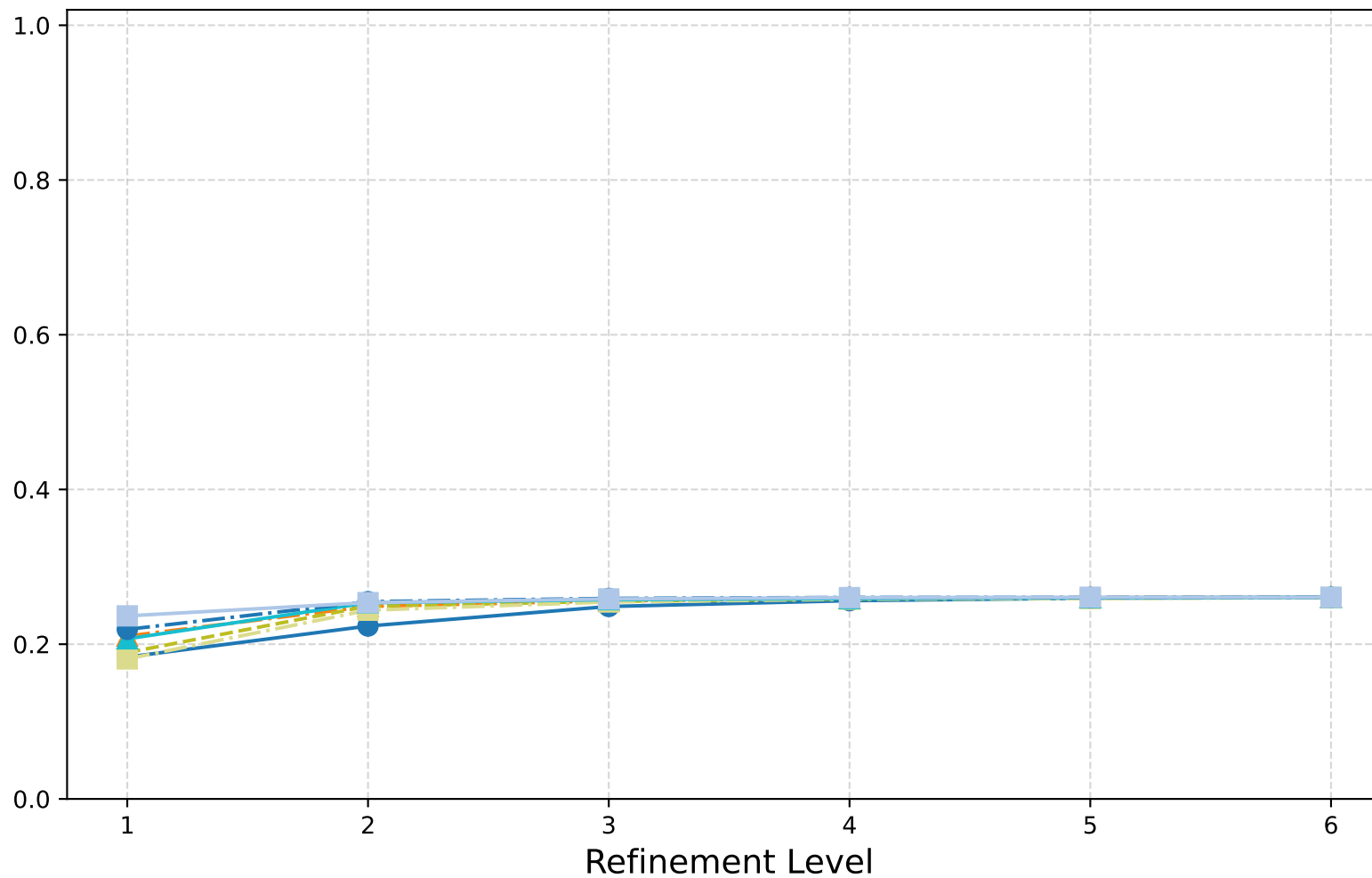
Dirac: W-Cycle (Scaled Id) - Spectral Radii
