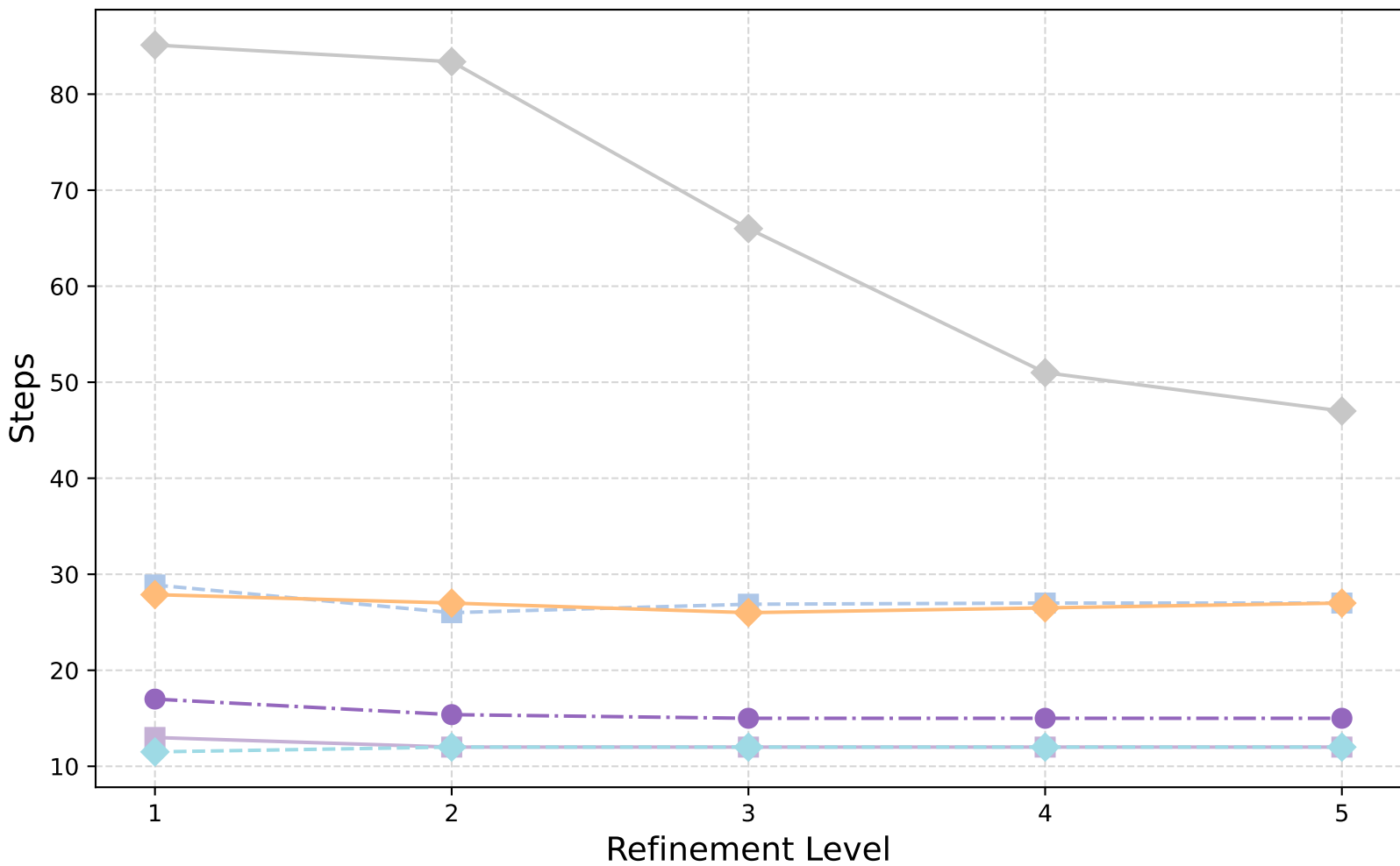
Dirac: W-Cycle (Scaled Id) - GMRES Iterations
