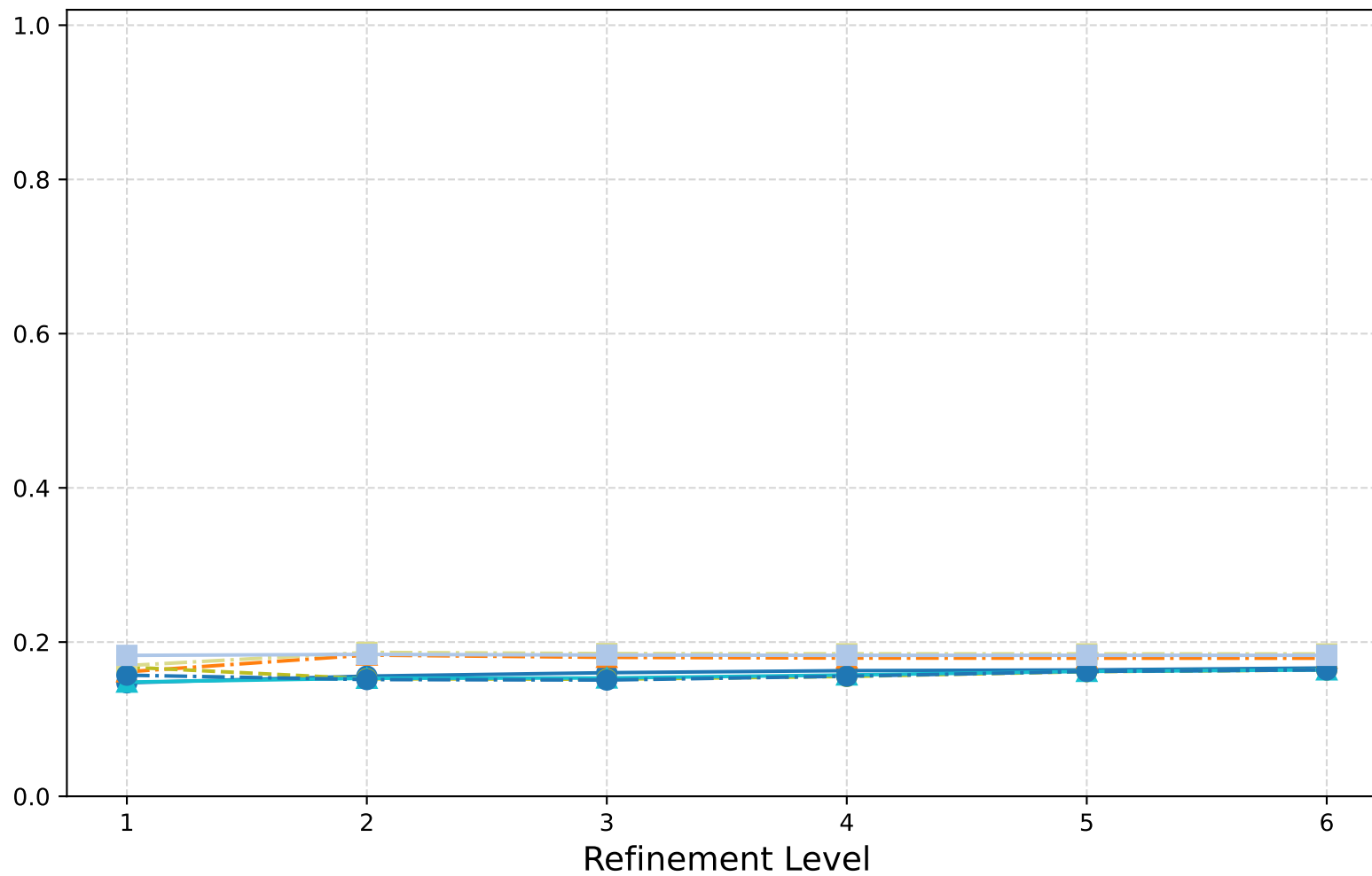
HCurl Laplacian: W-Cycle(Scaled Id) - Spectral Radii
