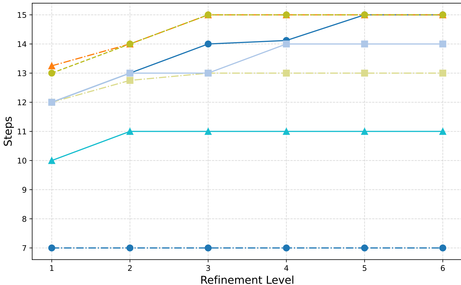
HCurl Laplacian: W-Cycle (Scaled Id) - GMRES Iterations
