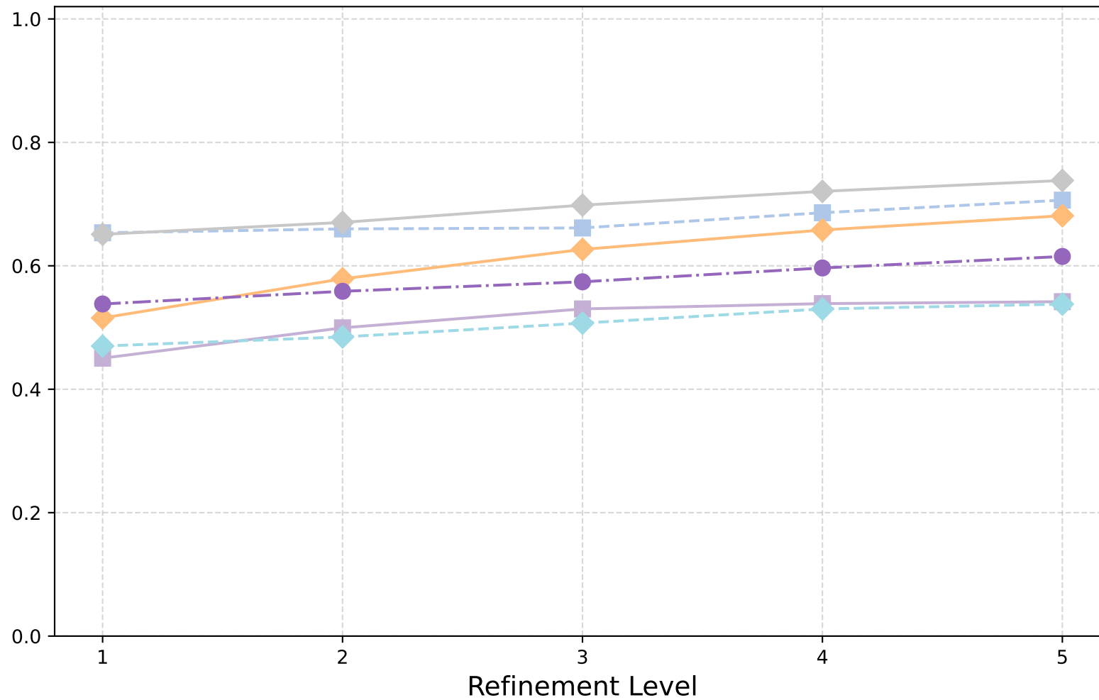
Dirac: V-Cycle (Barycentric) - n_{\text{ev}} -largest EV (mag.)
