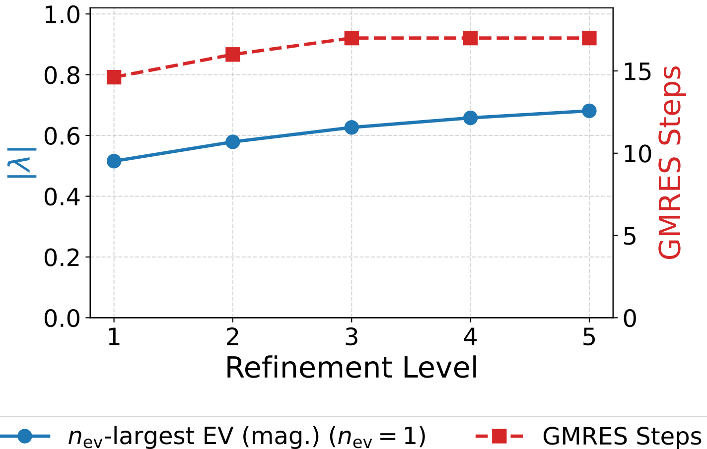
Dirac: V-Cycle (Barycentric)
