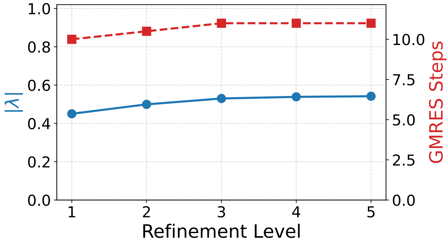
Dirac: V-Cycle (Barycentric)
