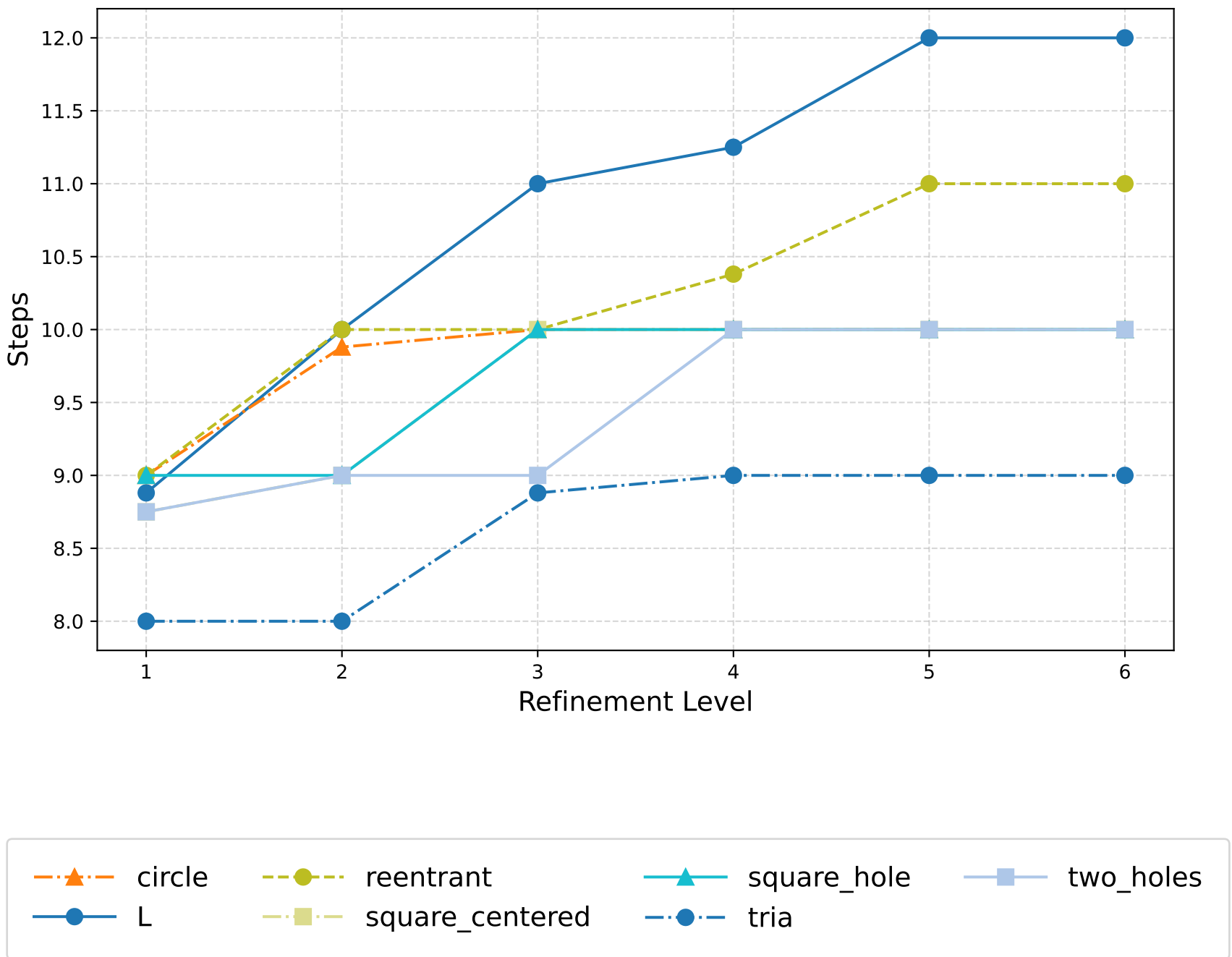
Magnetostatics: V-Cycle (Barycentric) - GMRES Iterations
