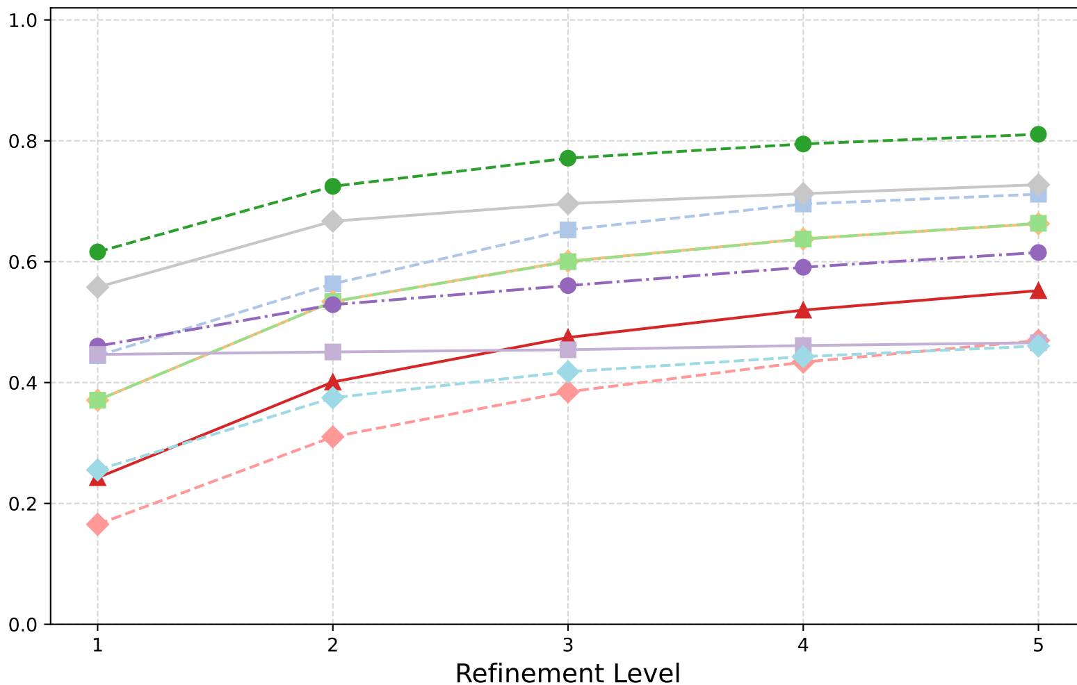
Magnetostatics: V-Cycle (Barycentric) - n_{\text{ev}} -largest EV (mag.)
