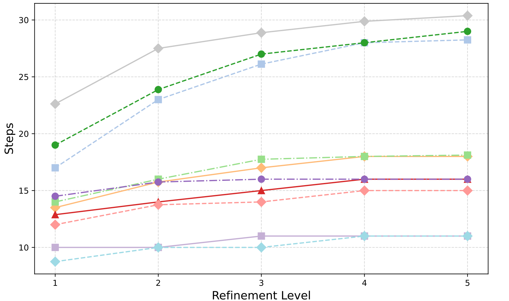
Magnetostatics: V-Cycle (Barycentric) - GMRES Iterations
